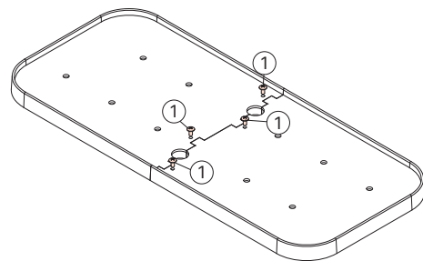
1. M4x8 screw
