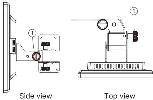
1. Manual screw
